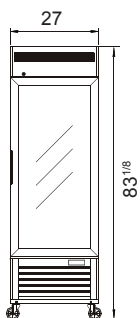
MCF8705GR
